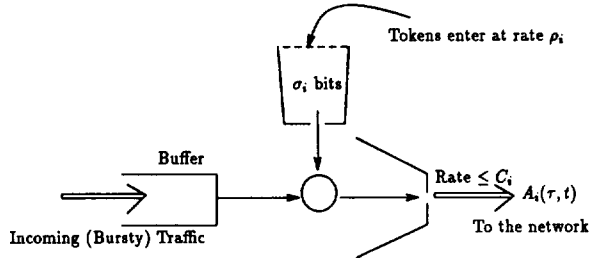
Fig. 3. A Leaky Bucket.
