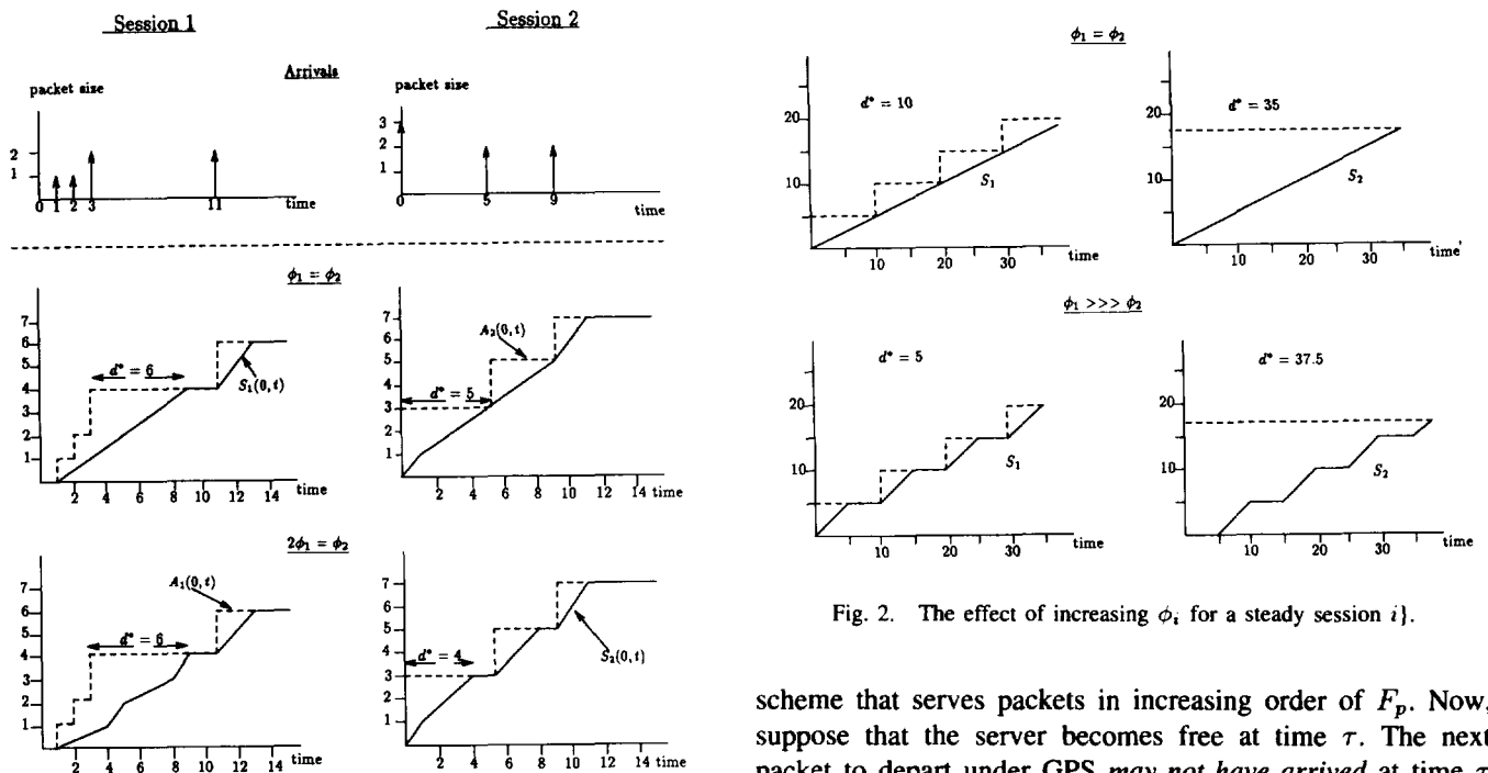
Fig. 1. An example of generalized processor sharing.
