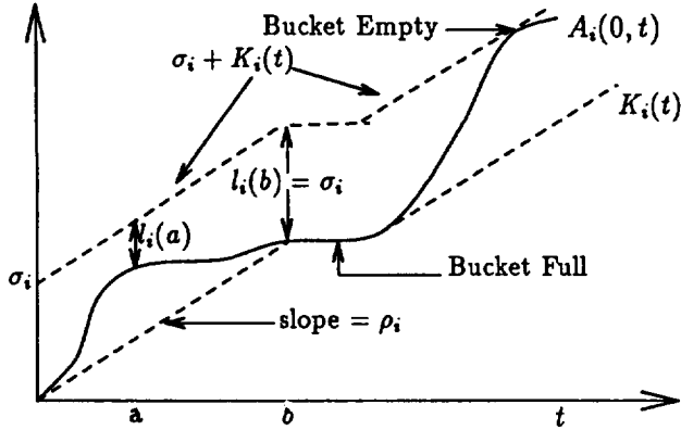
Fig. 4. A_i(t) and l_i(t) .
