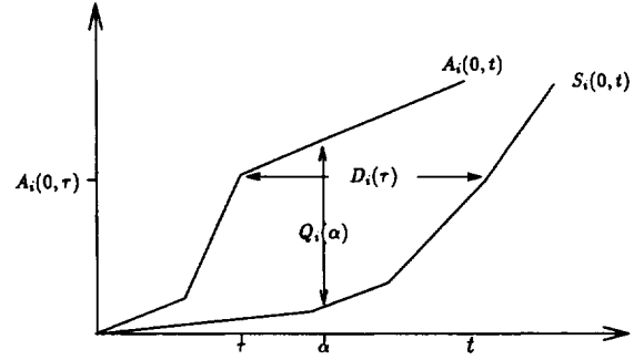
Fig. 5. A_i(0, t) , S_i(0, t) , Q_i(t) and D_i(t)
